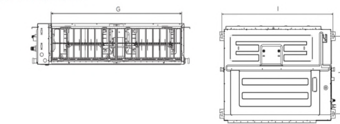
Air inlet dimensions
