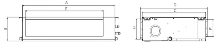
Air inlet dimensions
