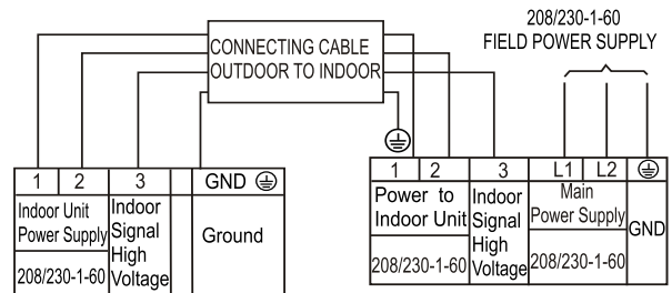
Fig. 7 — Connection Diagram 208/230V
