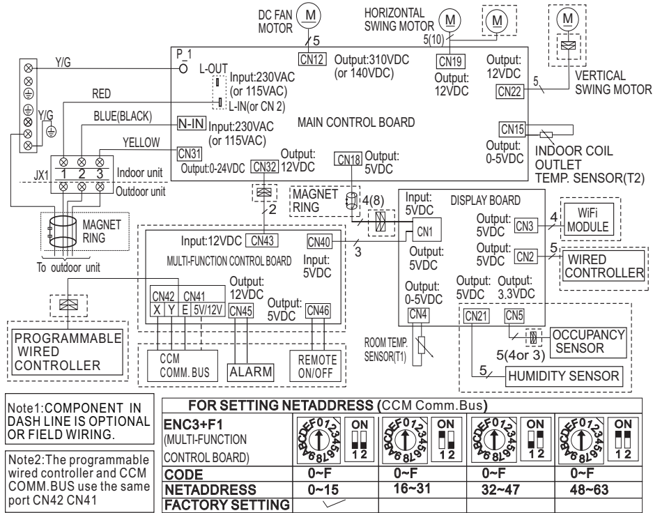
Fig. 5 — Wiring Diagram Sizes 6K - 36K (115V and 208/230V)
