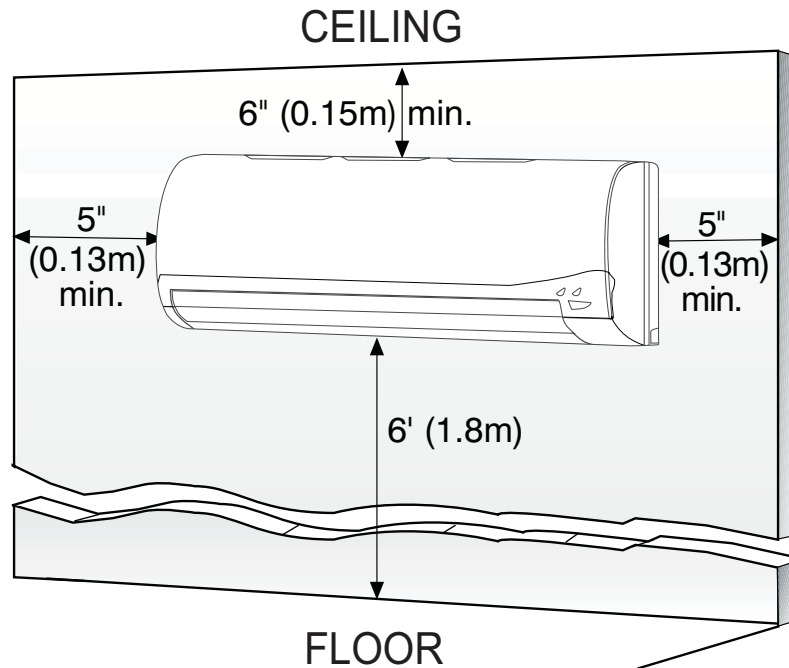
Fig. 2 — Indoor Unit Clearances
