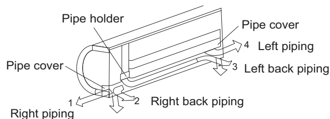
Fig. 3 — Piping Locations
