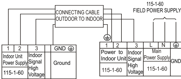
Fig. 6 — Connection Diagram 115V
